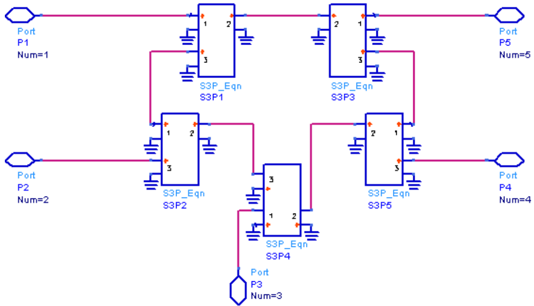
Figure 4-3 EQUATION BASED W-BCRCD SCHEMATIC Equation-Based, ideal Wilkons dividers linked together to create an ideal model for the W-BCRCD.
